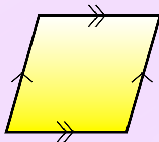
Rhombus 4 equal sides opposite sides are parallel opposite angles are equal
