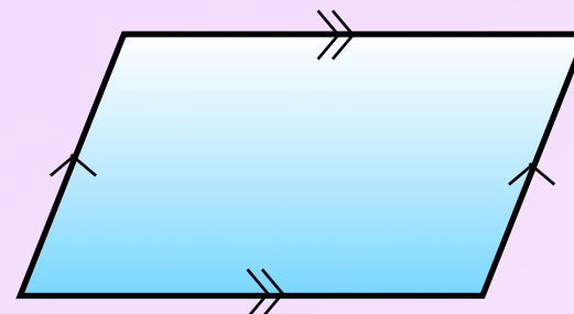
Parallelogram opposite sides are equal and parallel
