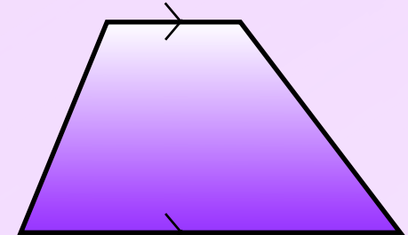
Trapezium 1 pair of parallel sides
