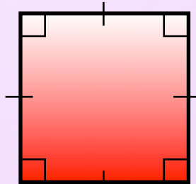
Square 4 equal sides 4 right angles
