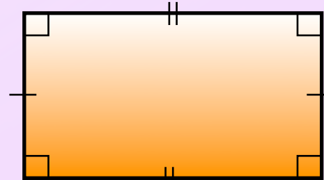
Rectangle opposite sides are equal 4 right angles
