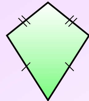
Kite 2 pairs of adjacent sides are equal
