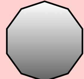
10 equal sides Regular Decagon
