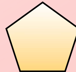
5 equal sides Regular Pentagon
