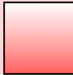
4 equal sides Regular Quadrilateral
