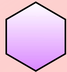
6 equal sides Regular Hexagon
