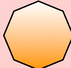
8 equal sides Regular Octagon
