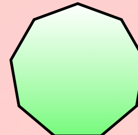
9 equal sides Regular Nonagon
