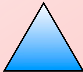
3 equal sides Regular Triangle
