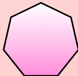
7 equal sides Regular Heptagon
