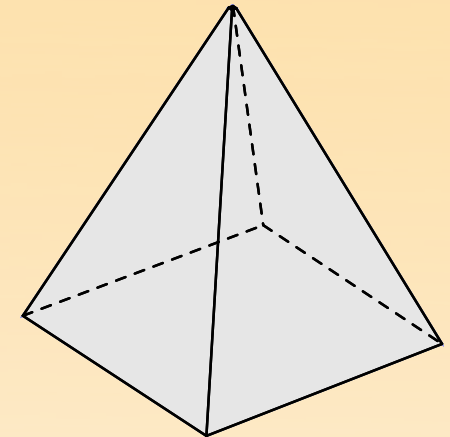
Square-based pyramid
