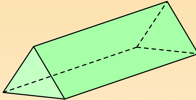
Triangular prism
