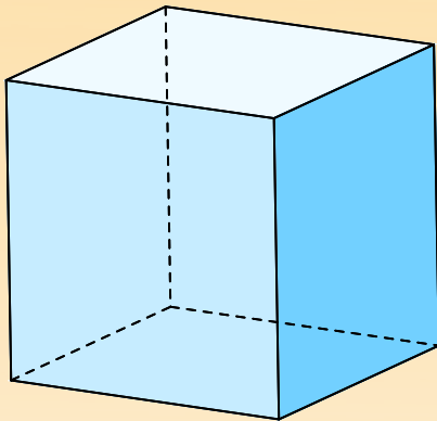
Cube
